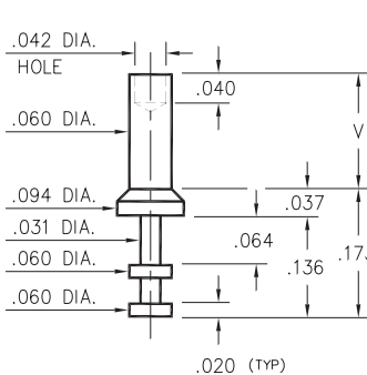
2317-X-00-XX-00-00-07-0 Swage mount in .064 hole
