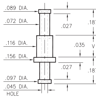
2708-X-00-XX-00-00-07-0 Swage mount in .120 hole
