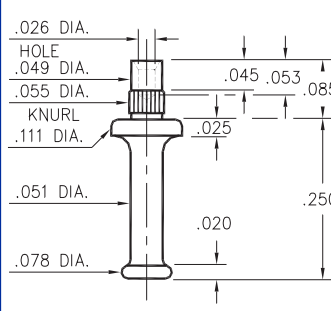
2533-0-00-XX-00-00-07-0 Press-fit & swage in .052 mtg. hole. For .062 thick board
