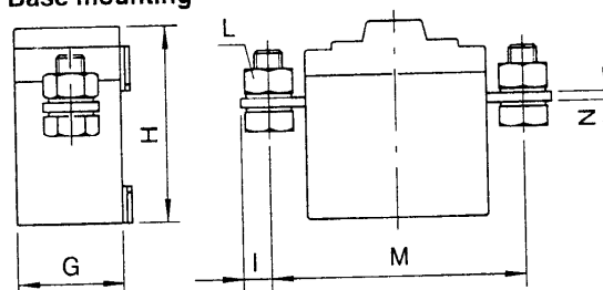
Base mounting
