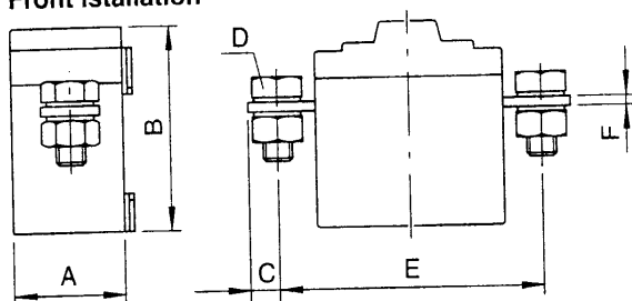
Front installation
