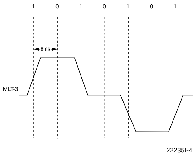
Figure 2. MLT-3 Waveform
