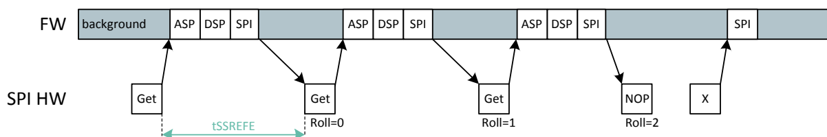
Figure 4 – Trigger Mode 1
