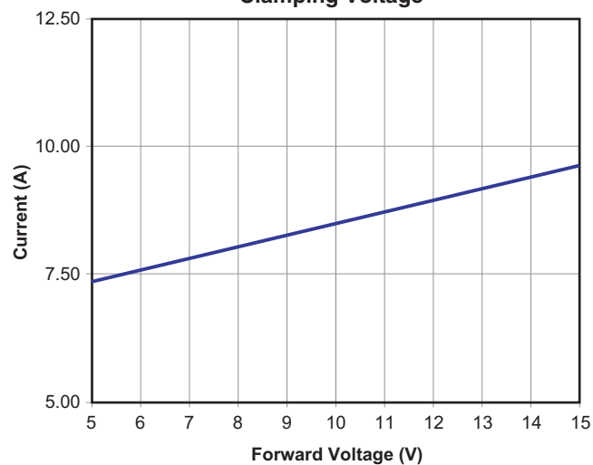
Clamping Voltage
