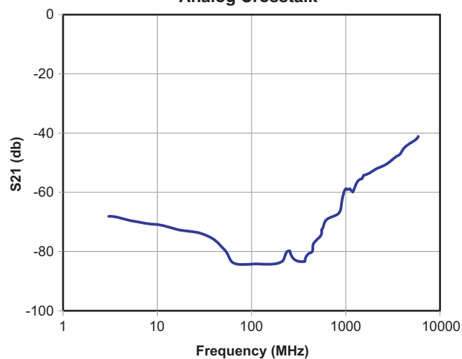
Analog Crosstalk
