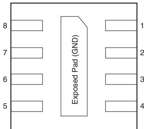
DFN-8 (Bottom View)
