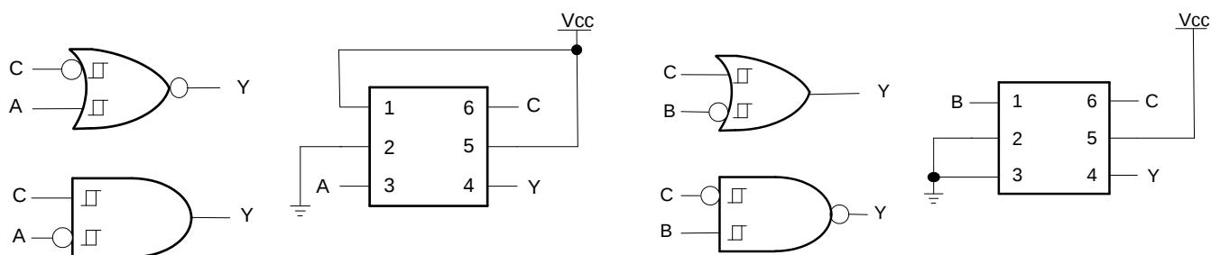
Configuration 4 2-Input OR Gate with One Input Inverted 2-Input NAND Gate with One Input Inverted
