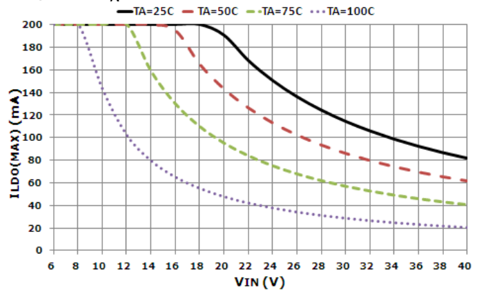
FIGURE 22. I LDO(MAX) vs V IN
