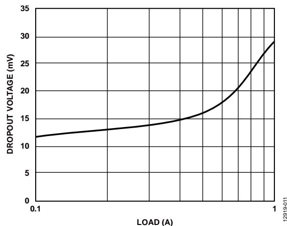
Figure 11. Dropout Voltage vs. Load Current, V_{\text{OUT}} = 1.3 \text{ V}
