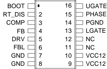
SSOP-16
