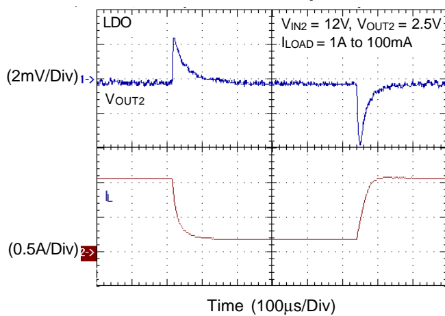
Transient Response
