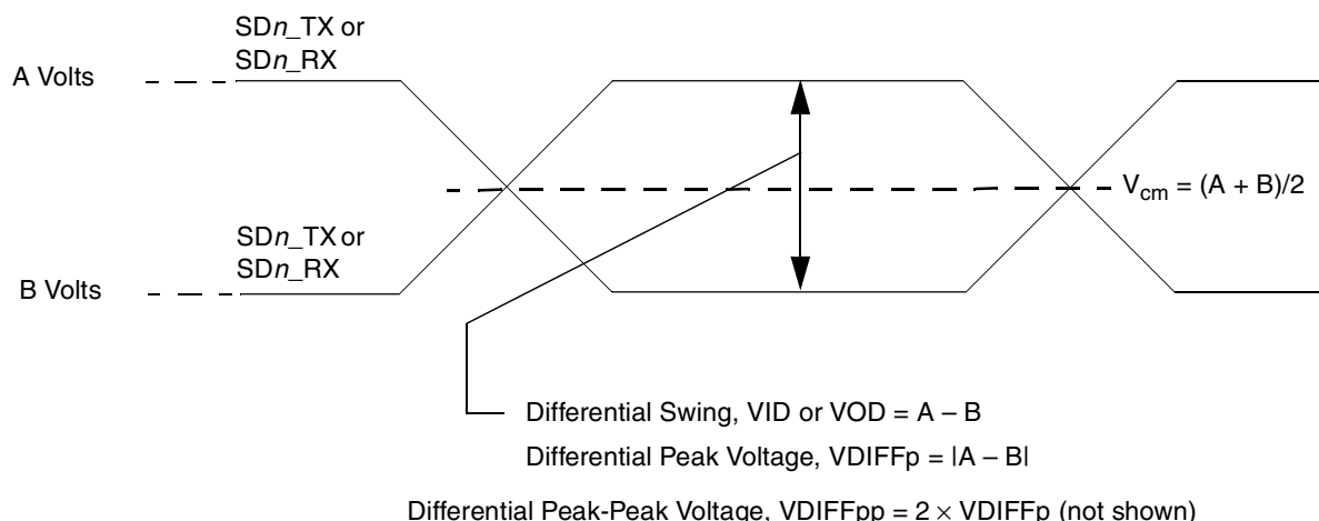
Figure 48. Differential Voltage Definitions for Transmitter or Receiver
