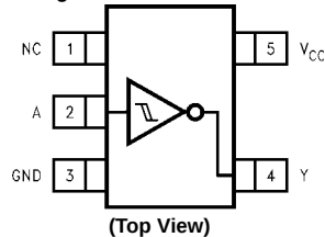
Pad Assignments for MicroPak
