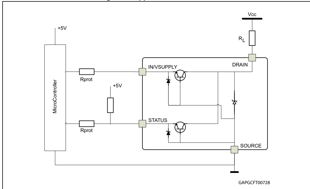
Figure 5. Application schematic
