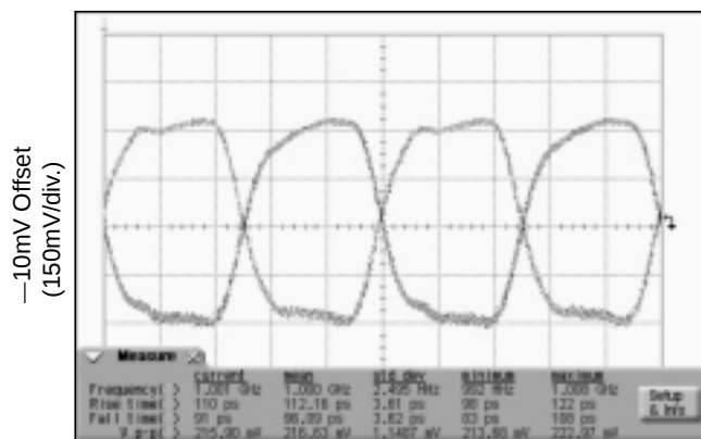
1GHz Output
