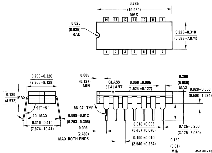
Cavity Dual-In-Line Package (J) Order Number LM119J, LM119J/883, LM219J, LM319AJ or LM319J NS Package Number J14A
