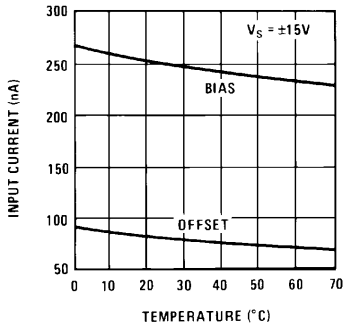
Input Currents
