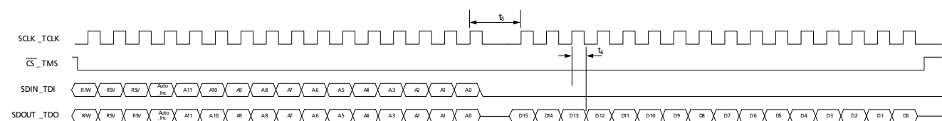
Figure 4-29: Read Mode
