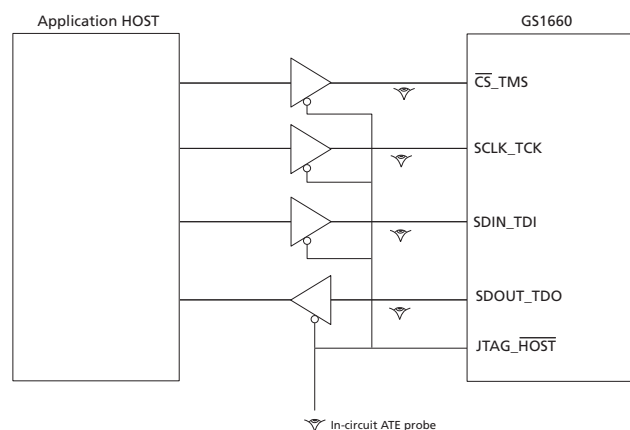
Figure 4-31: In-Circuit JTAG
