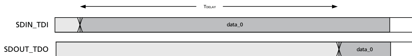
Figure 4-30: GSPI Time Delay
