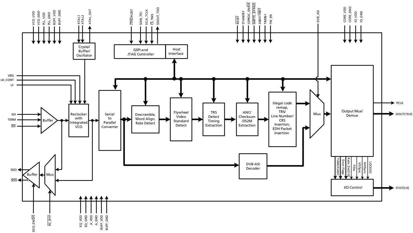
GS1660 Functional Block Diagram
