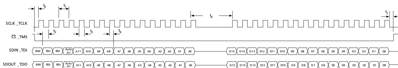
Figure 4-28: Write Mode
