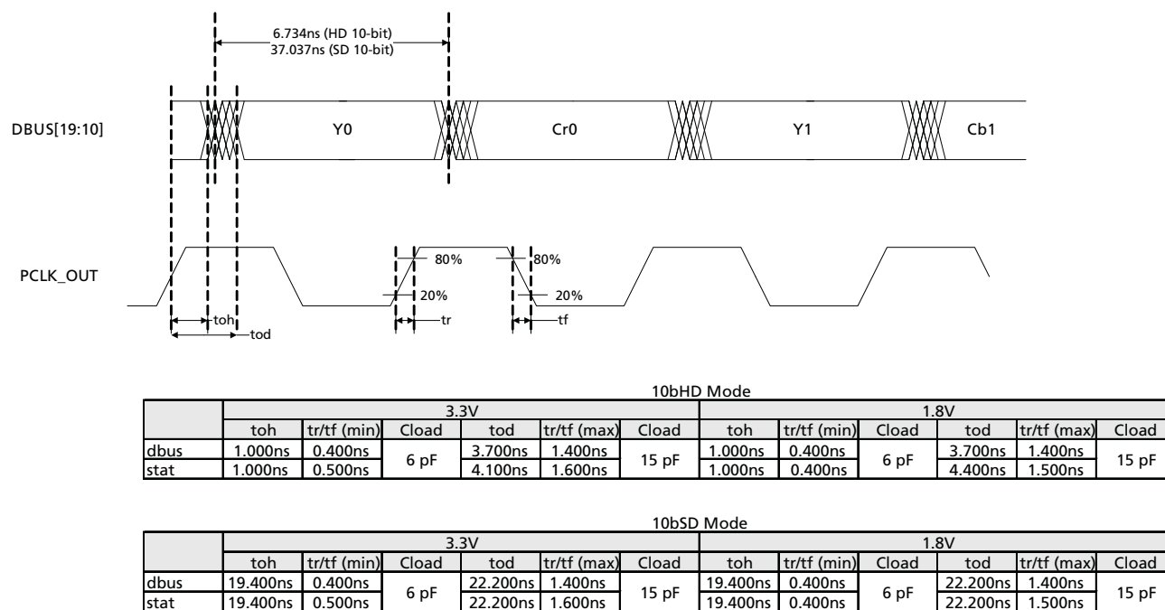
Figure 4-2: PCLK to Data and Control Signal Output Timing - SDR Mode 1
