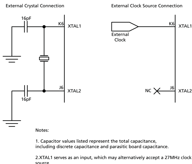
Figure 4-1: 27MHz Clock Sources
