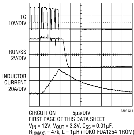
Short-Circuit Test
