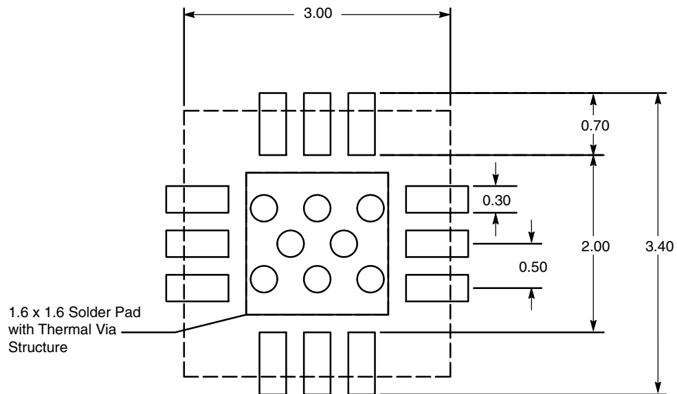
Figure 21. PCB Pad Layout for QFN 3 × 3
