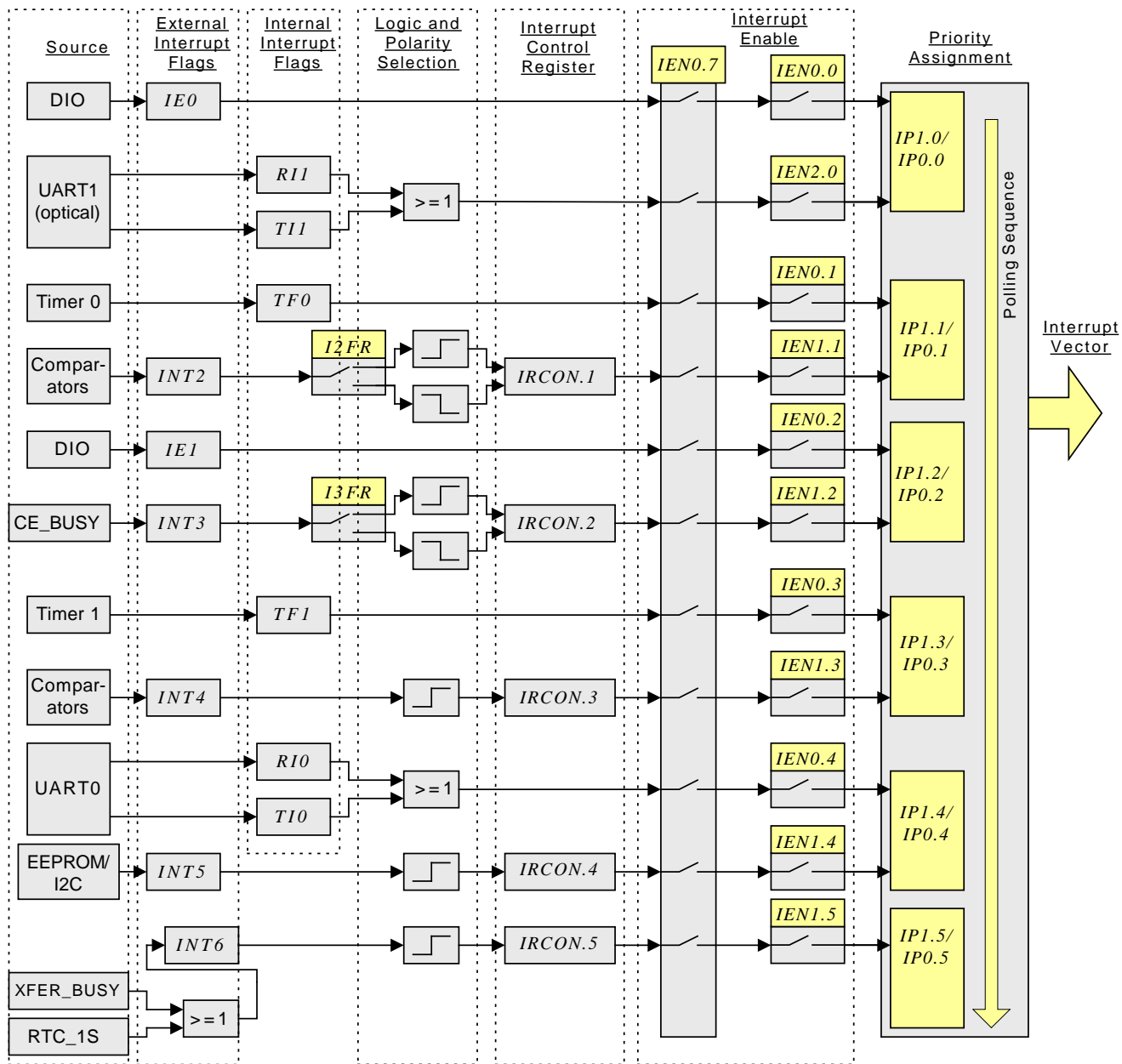
Figure 7: Interrupt Structure
