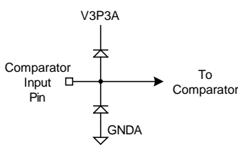
Comparator Input Equivalent
