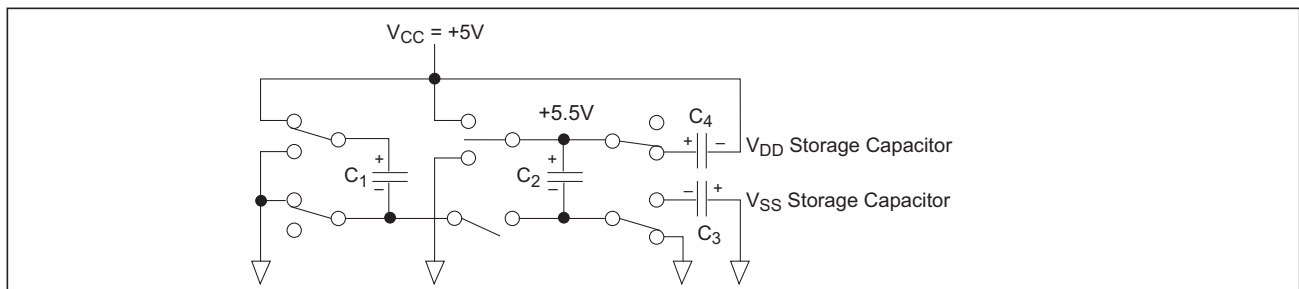
Figure 17. Charge Pump — Phase 4
