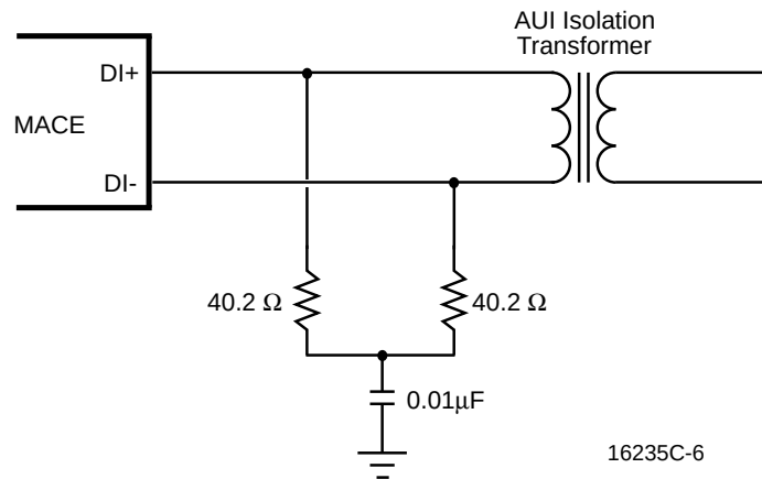
Differential Input Termination
