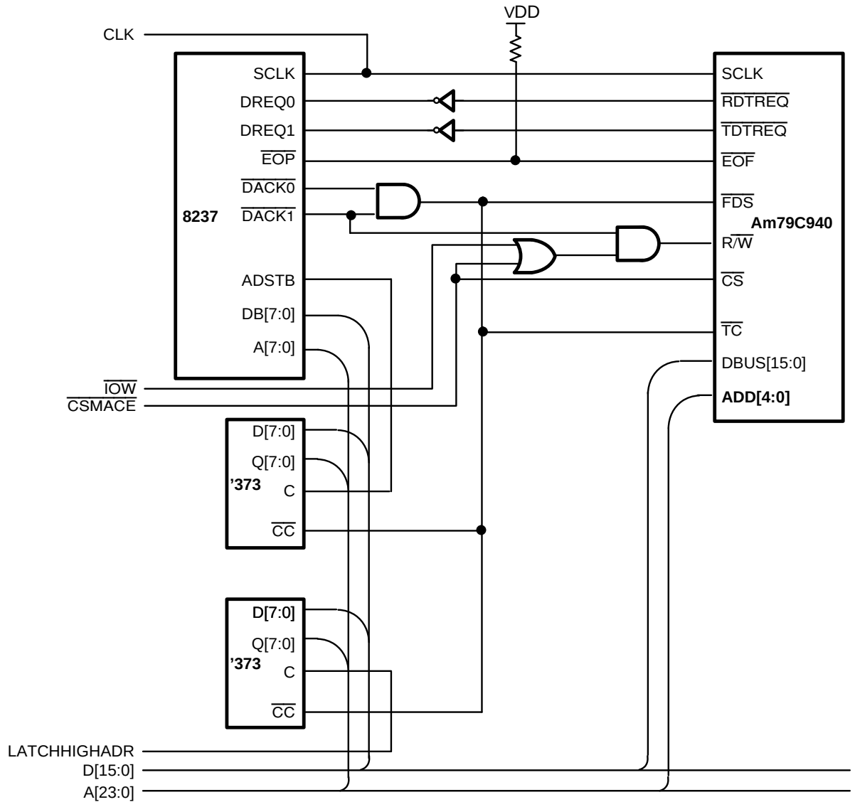
System Interface – Motherboard DMA Example
