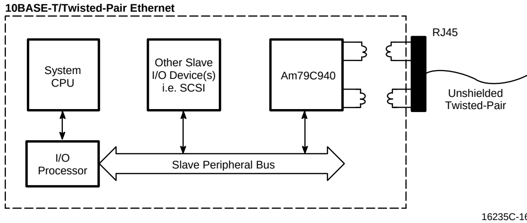
AUI-10BASE-T/Unshielded Twisted-Pair Interface
