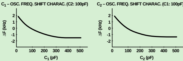
Figure 7: Load Capacitor Effects
