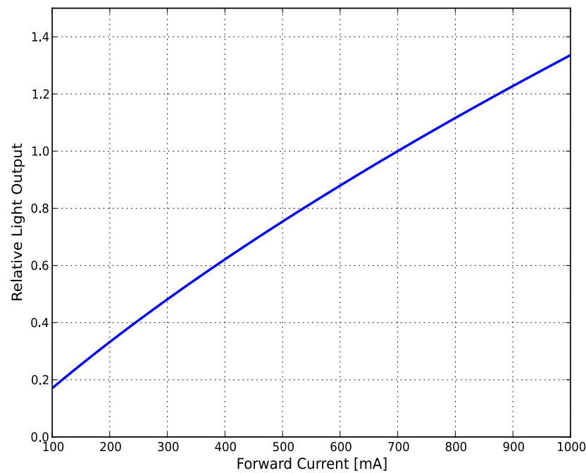
Figure 2b: Typical normalized light output vs. forward current for LXFx-FWxx at T j =85°C.
