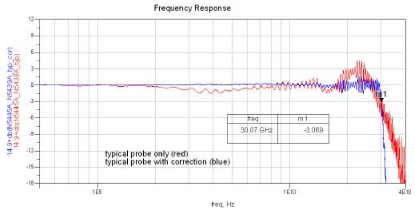
Frequency response plot with 1 mm span
