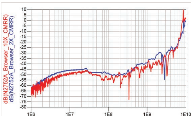
Common mode rejection ratio (red= 2:1, blue= 10:1)
