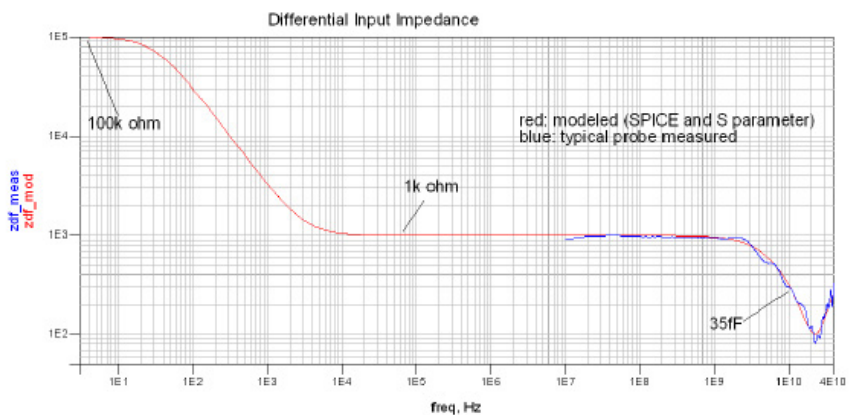
Differential input impedance
