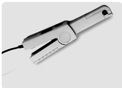
1146B 100 mA to 100 Arms, dc to 100 kHz probe.
