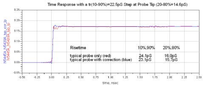
Time domain response plot with 1 mm span
