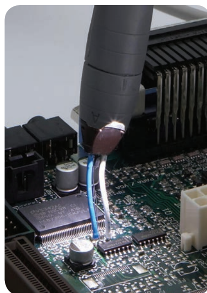
N2750A with solder-in tip
