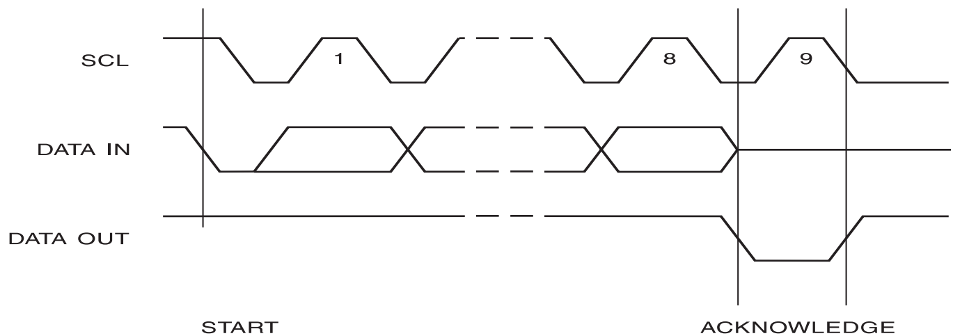
Figure 6. Output Acknowledge
