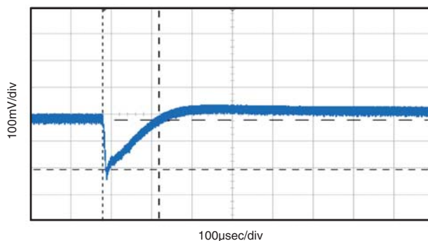
UCQ-3.3/30-D48 Output Transient Response ( V_{IN} = 48V , resistive load step 50% to 75%)
