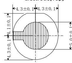
Electrode(Bottom) of 30MHz
