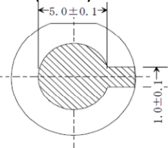
Electrode(Bottom) of 9MHz
