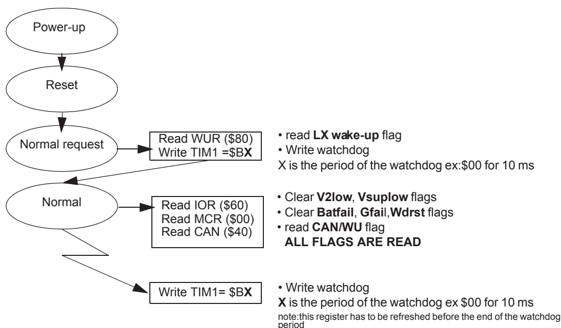
Figure 47. Normal Mode After Power-up
