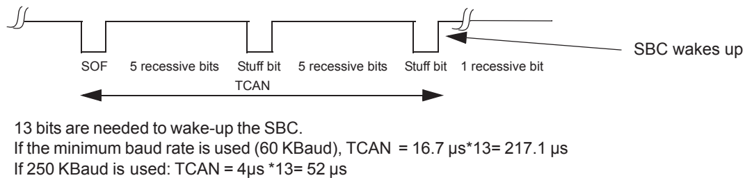
Figure 42. CAN Frame with 11 Bits of Identifier Field at 1
