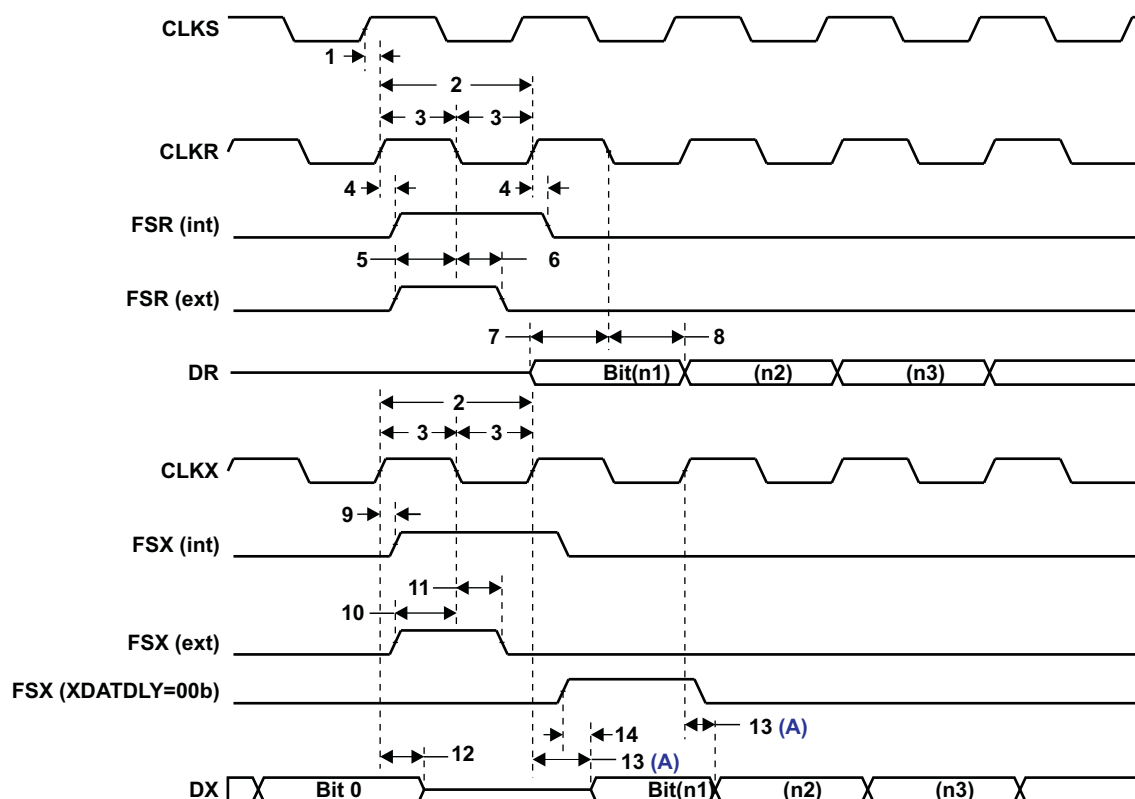
Figure 5-33. McBSP Timing
