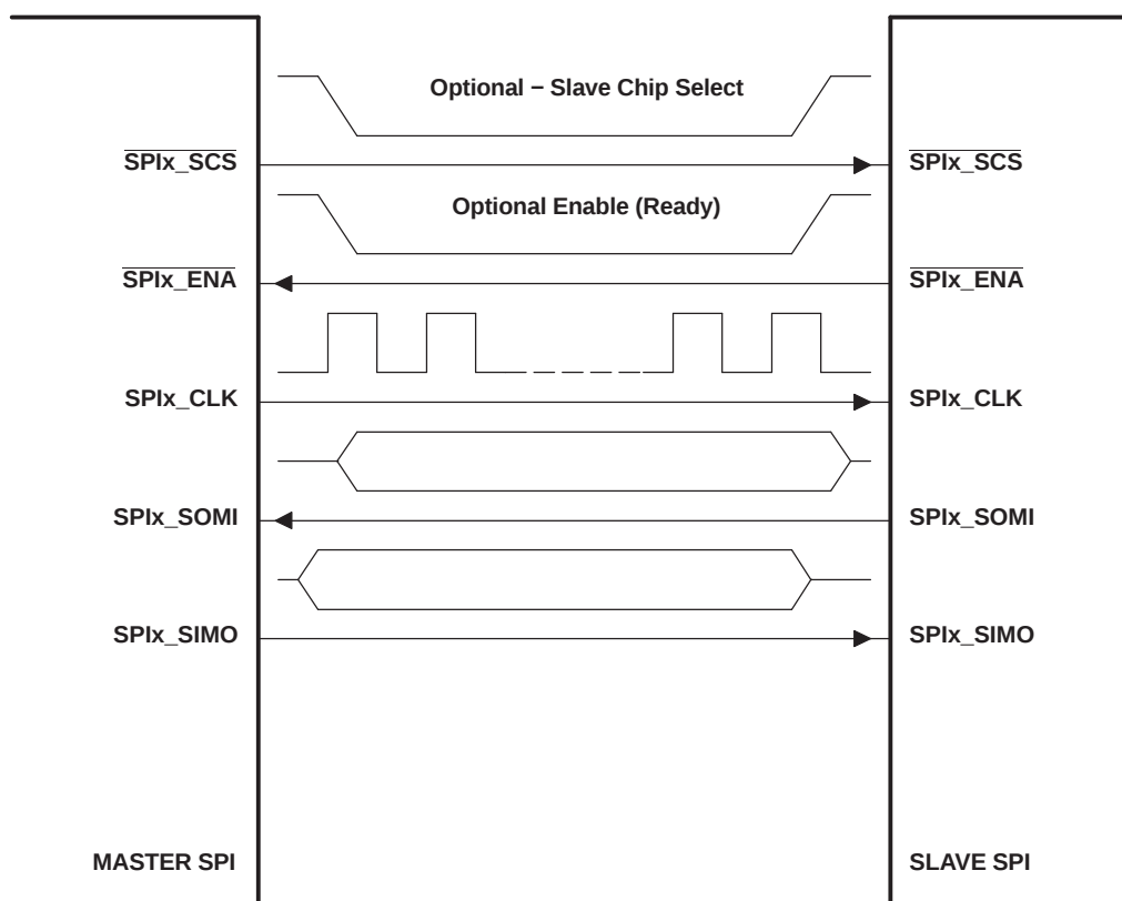
Figure 5-36. Illustration of SPI Master-to-SPI Slave Connection
