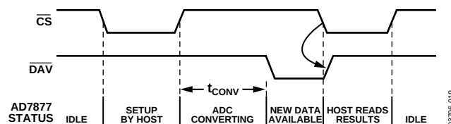
Figure 40. Operation of \overline{\text{DAV}} Output
