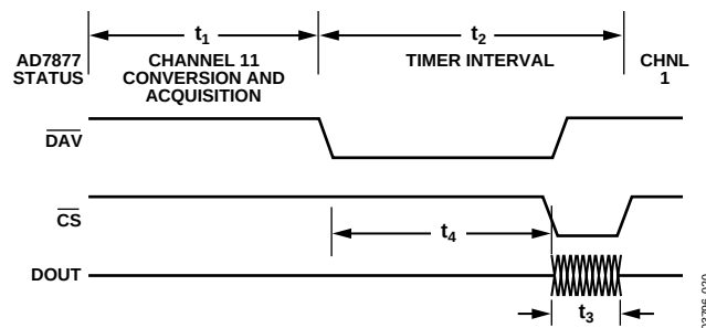
Figure 41. Timing for Reads after \overline{\text{DAV}} Goes Low
