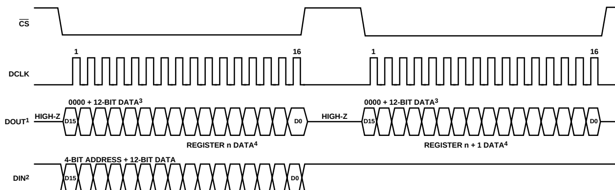
Figure 45. Designation of Data-Word Bits in AD7877 Write Operations
