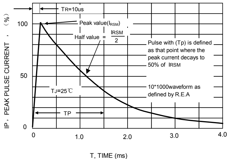
FIG.5 -PULSE WAVEFORM
