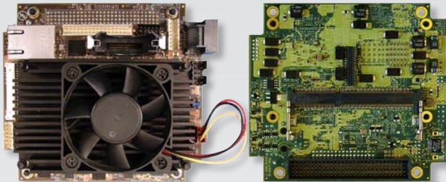
VL-EPMp-34S (Top)
