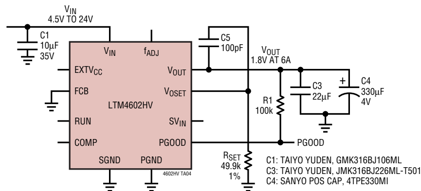
1.8V, 5A Regulator
