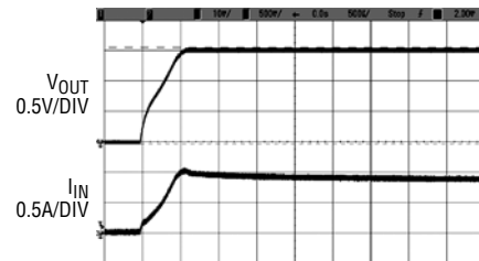
Start-Up, I_{OUT} = 6A (Resistive Load)
