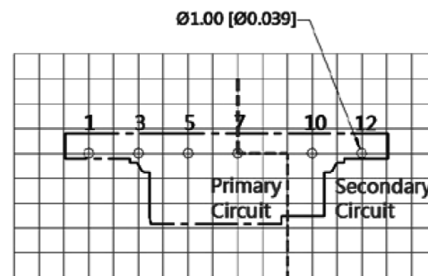
Top View PCB Layout
