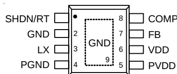
SOP-8 (Exposed Pad)
