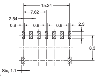
Mounting Dimensions (Top View) Tolerance: \pm 0.1 mm
