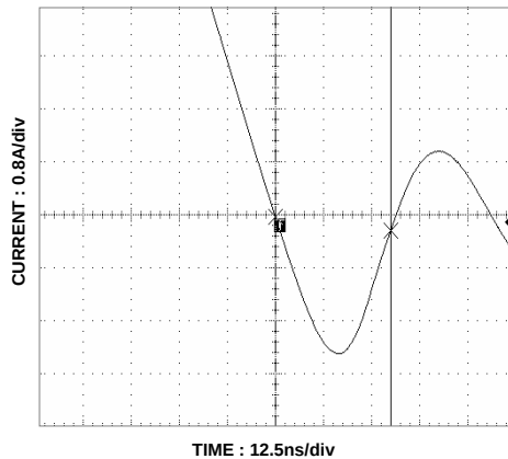
Figure 12. FDS6689S SyncFET body diode reverse recovery characteristic.
