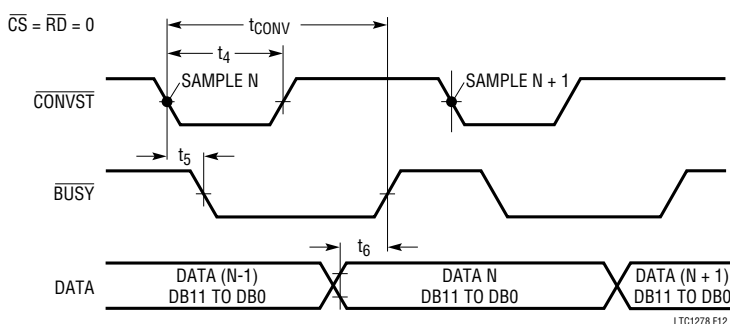
Figure 12. Mode 1a. \overline{CONVST} Starts a Conversion. Data Outputs Always Enabled. ( \overline{CONVST} = \text{low pulse} )
