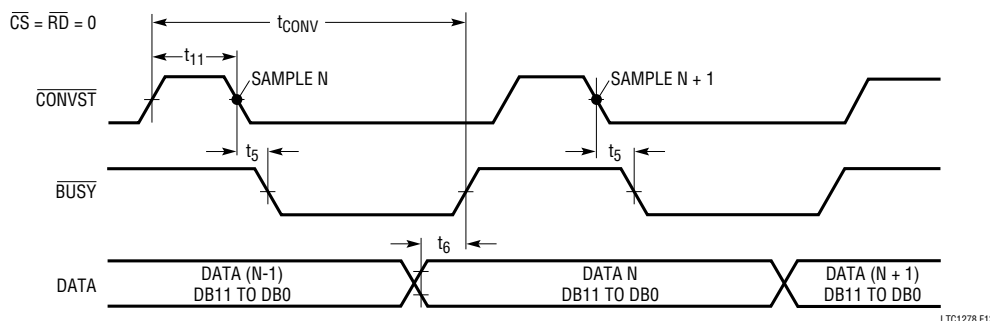
Figure 13. Mode 1b. \overline{CONVST} Starts a Conversion. Data Outputs Always Enabled. ( \overline{CONVST} = \text{high pulse} )
