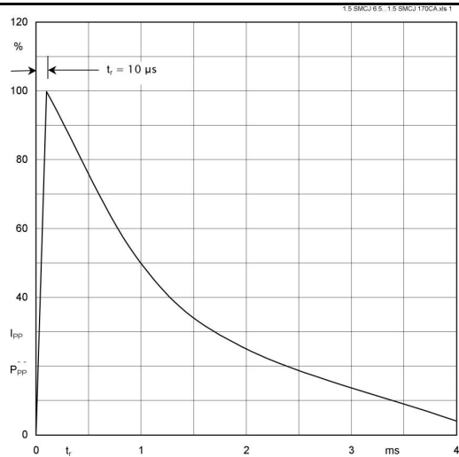
Fig. 1 10/1000 \mu s - pulse waveform
