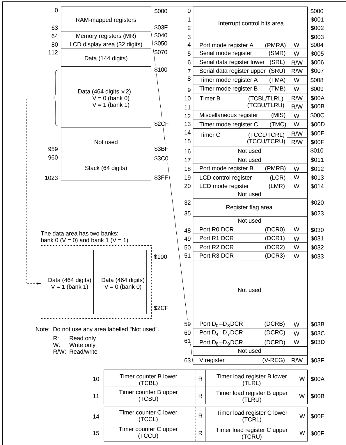
Figure 2 RAM Memory Map (1,184-digit × 4-bit)
