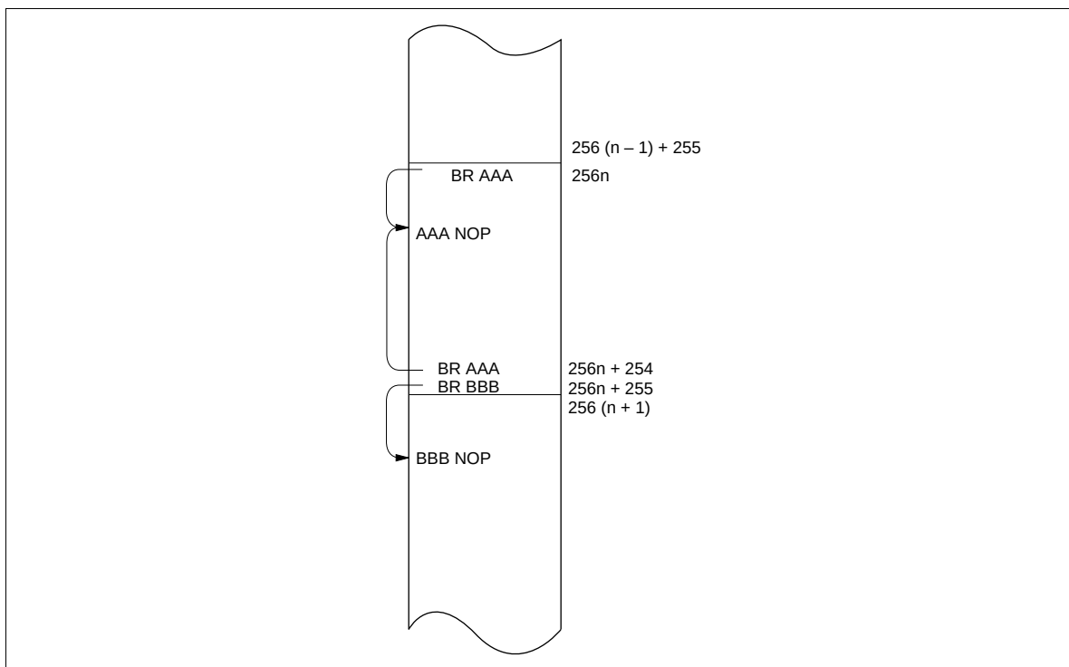
Figure 41 Page Boundary between BR Instruction and Branch Destination
