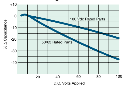
Voltage Coefficient
