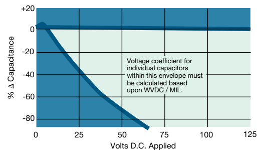
Voltage Coefficient
