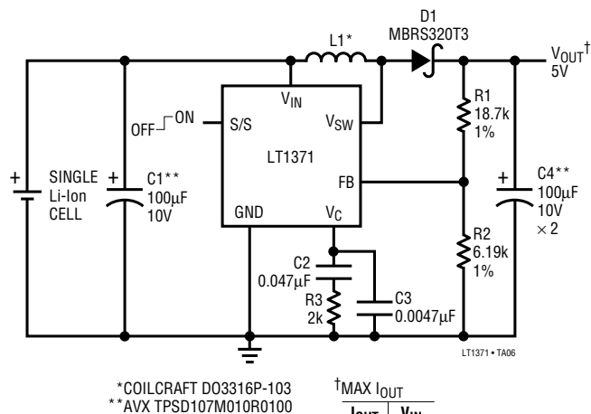
Single Li-Ion Cell to 5V
