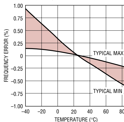
Frequency Error vs Temperature
