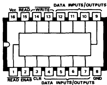
C31 DM8553N 8-bit latch (Tri-state)
