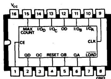
C27 DM8512N Dual Gated Master Slave JK/D Flip Flop
