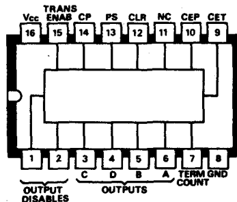
C30 DM8552N Decade counter/latch (Tri-state)
