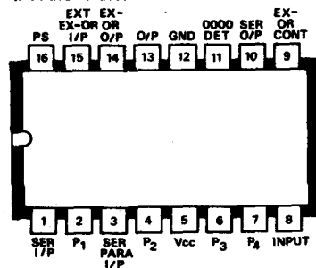
C28 DM8520N Modulo-N-divider
