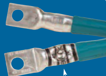
Lower Side of Connector with HEX-FLEX™ Crimp
