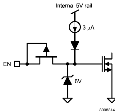
FIGURE 4. Enable Circuit
