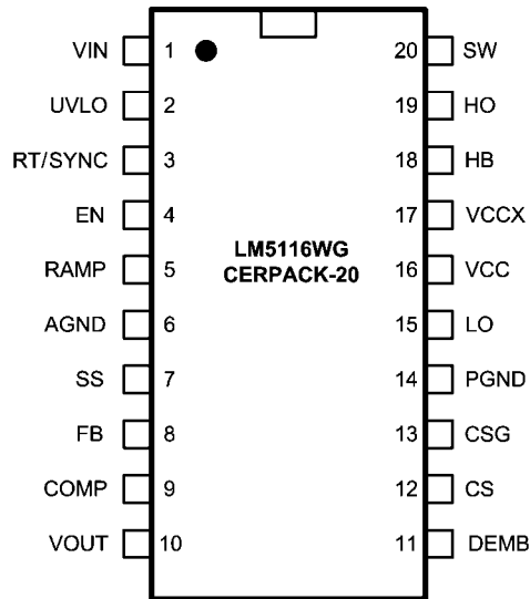
Top View See NS Package Number WG20A
