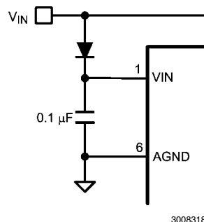
FIGURE 3. Input Blocking Diode for VCCX > VIN
