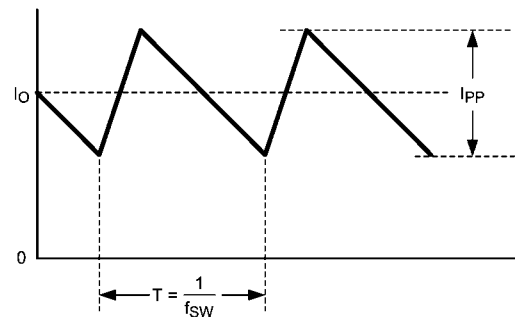
FIGURE 10. Inductor Current
