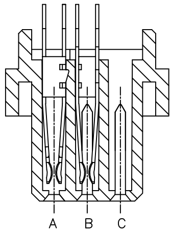
SECTION X-X ACCORDING TO 75948-X02
