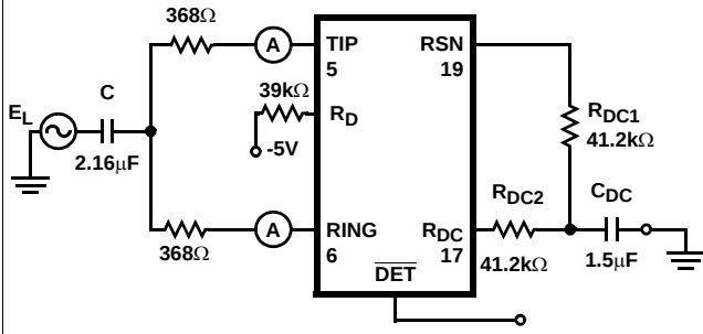
FIGURE 3A. OFF-HOOK
