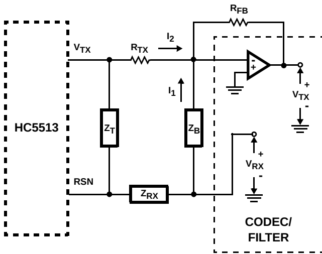
FIGURE 17. TRANSHYBRID CIRCUIT
