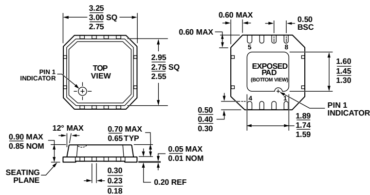
Figure 44. 8-Lead Frame Chip Scale Package [LFCSP_VD]
