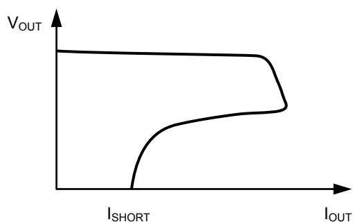
Figure 12 V_{\text{OUT}} vs. I_{\text{OUT}} Characteristics
