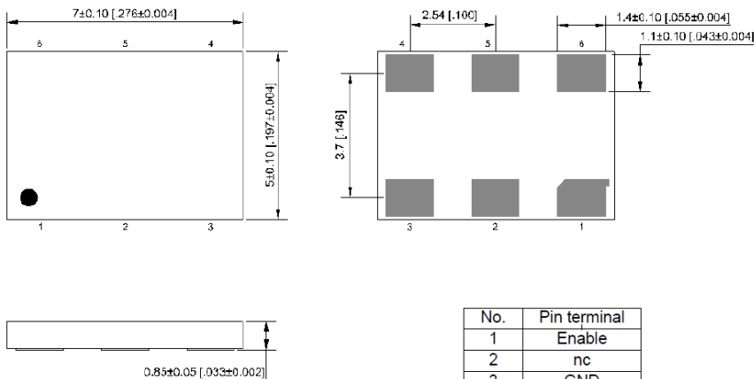
External Dimensions
